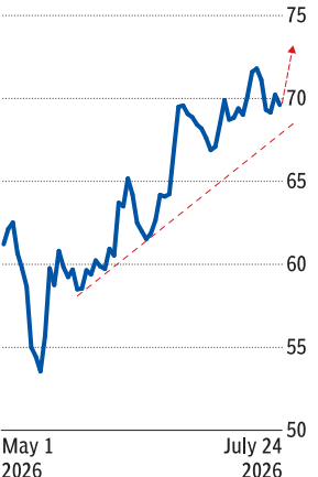
Gold/Silver ratio
